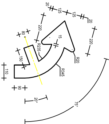
W2-10B(L) 750 x 750
