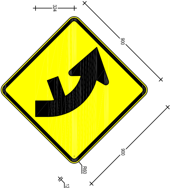
W2-10C(L) 900 x 900
