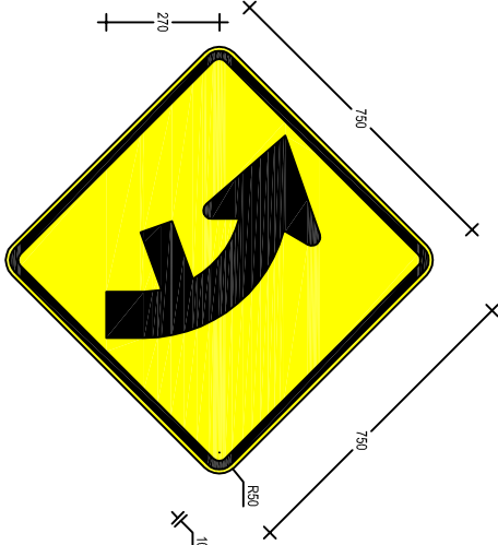
W2-10B(L) 750 x 750
